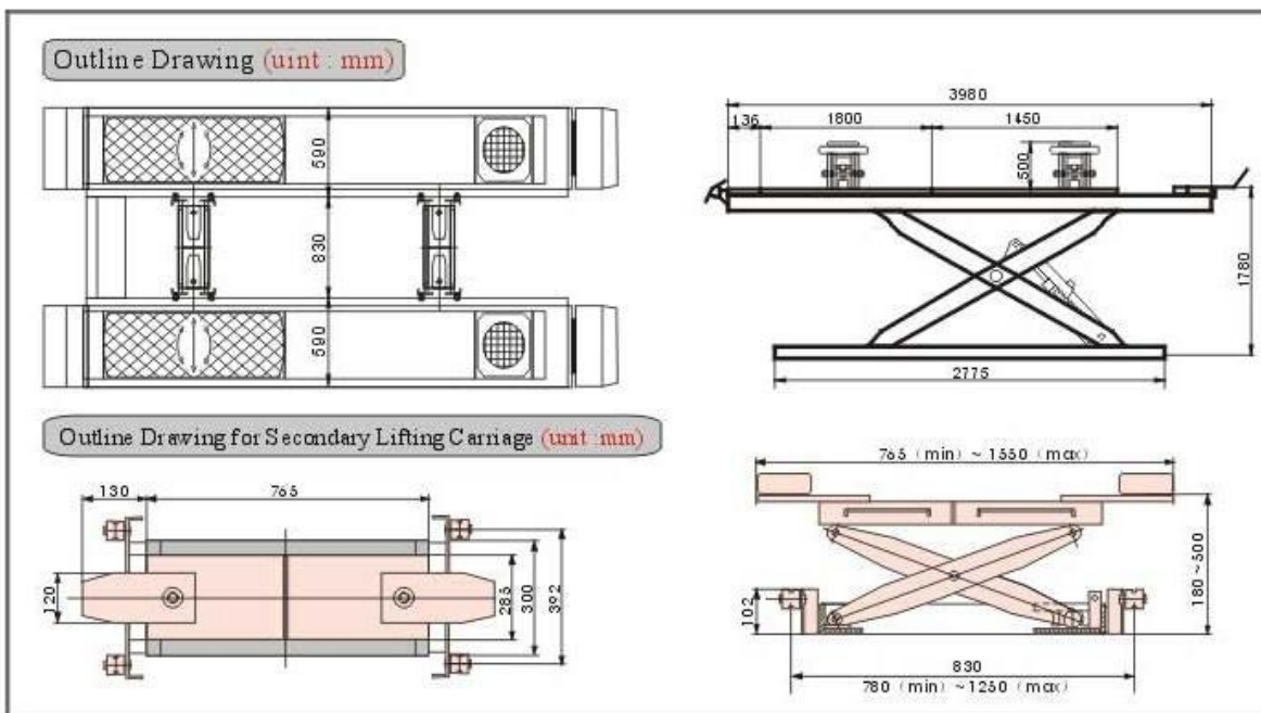
pneumatic double rack self lock safety security unit
